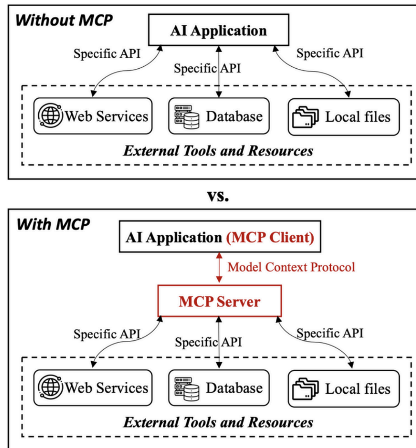
Figure 1: Tool invocation with and without MCP.
